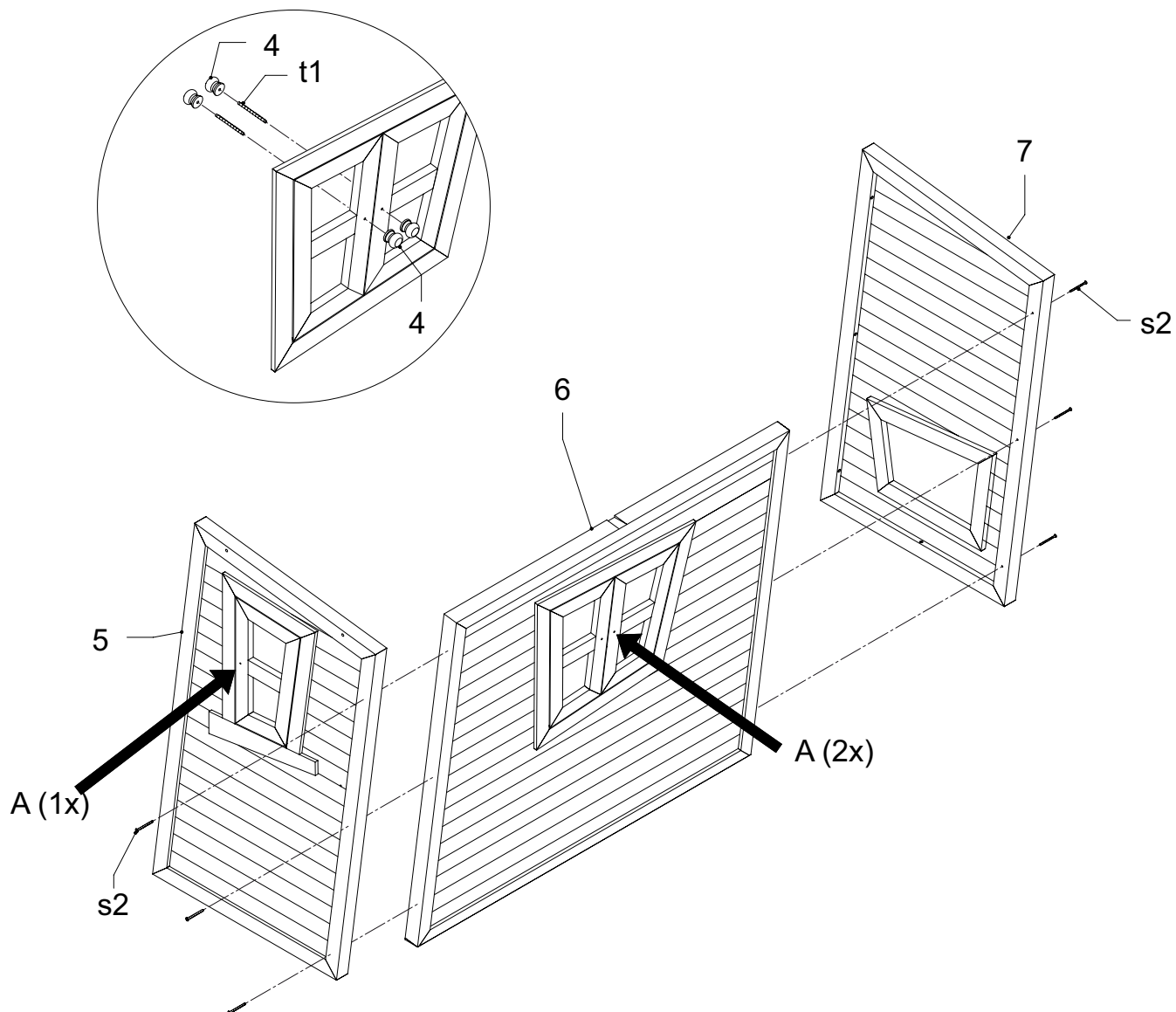
Detail A
